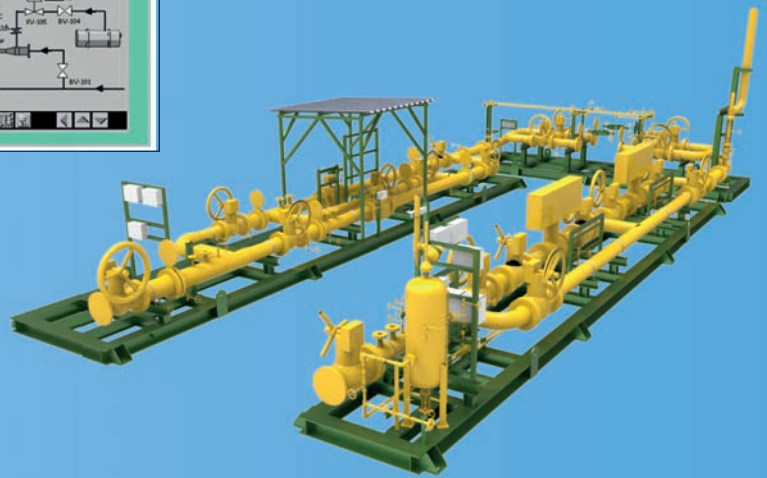
V.C.S. ® Vapor Condensing System suitable for gas phase condensing during tanks loading
