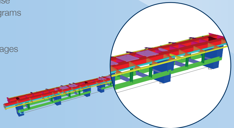
FEM analysis
