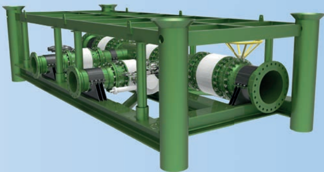
PLEM hydraulically operated
