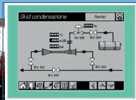
G.O.L.H. ® Gas On Line Heating system suitable for cryogenic LPG heating by sea water.
